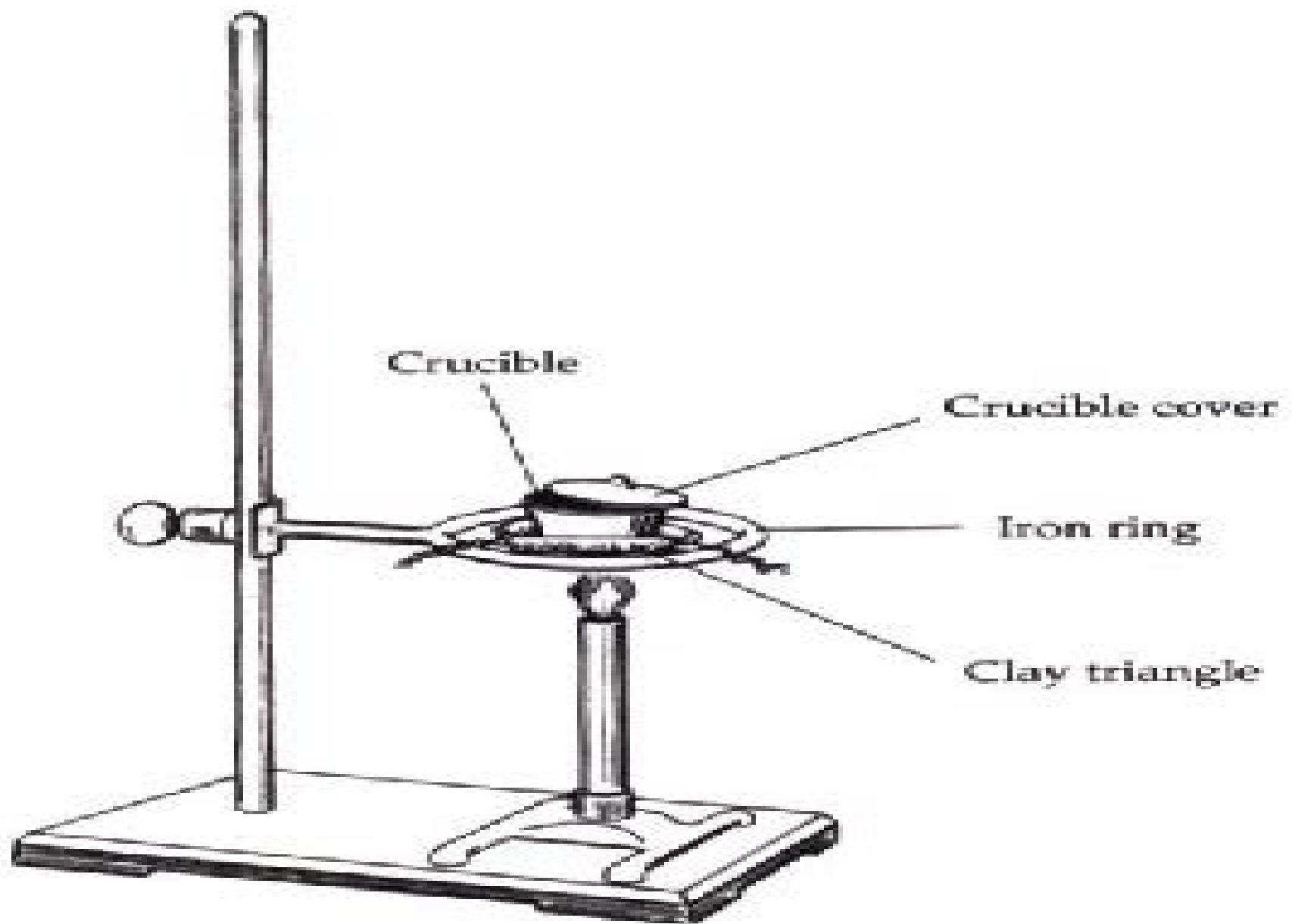
▲ FIGURE 5.2 Setup for copper sulfide determination.
