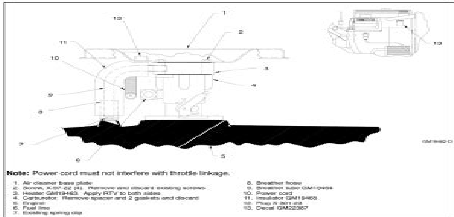
Figure 1 Carburetor Heater Assembly
