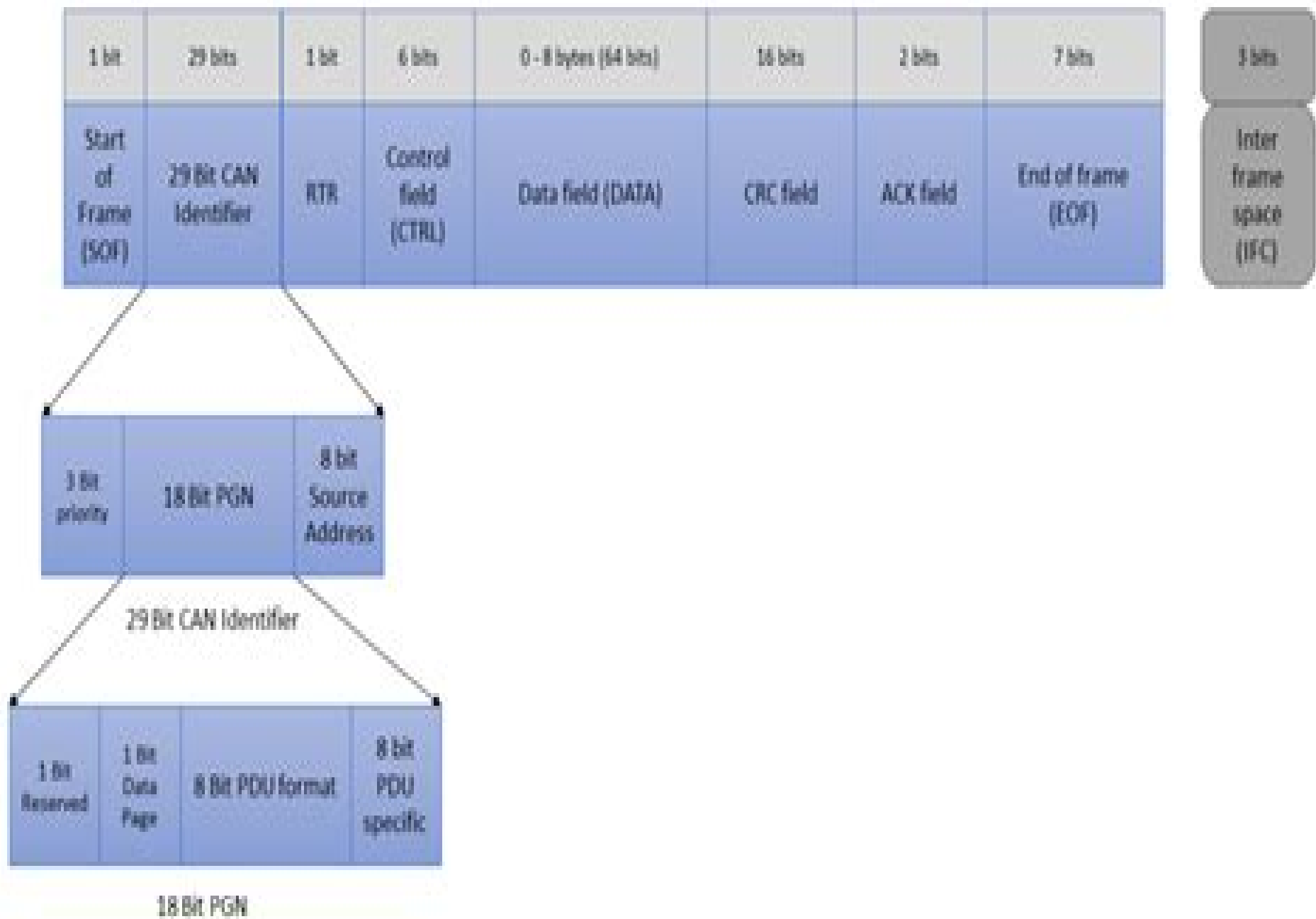
SAE J1939 CAN Frame structure
