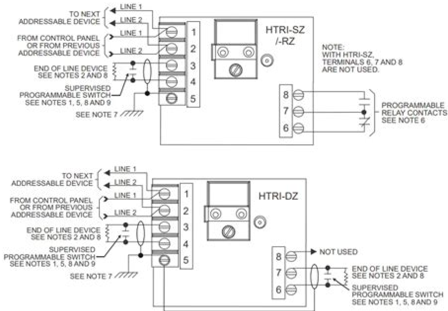
Figure 9 Security Point (1076) Wiring Connections
