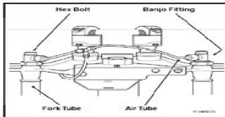
Figure 2-73. Banjo Bolt Cap Locations
