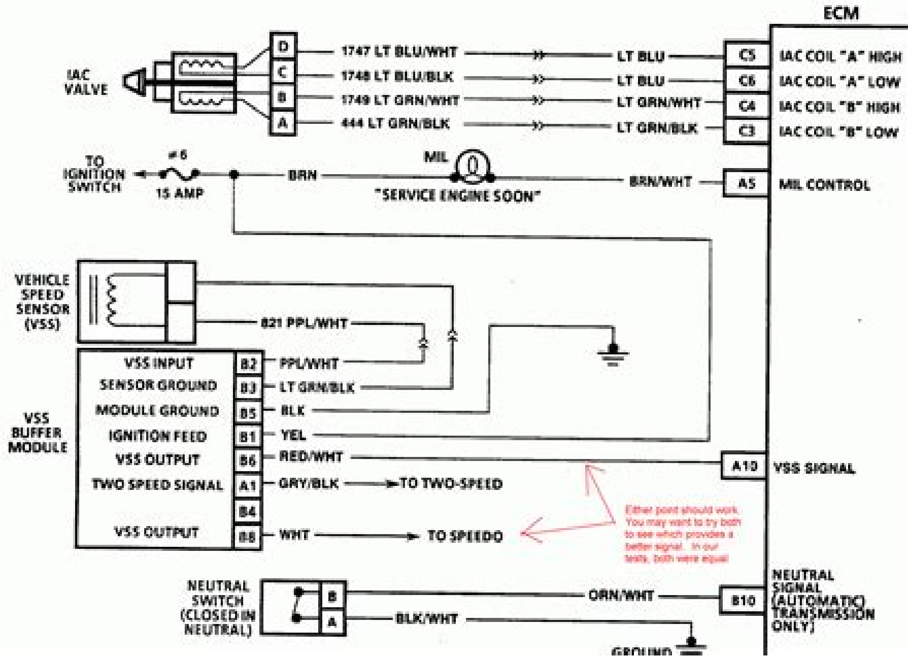
Figure 3-11 - ECM Wiring Diagram (2 of 3)
