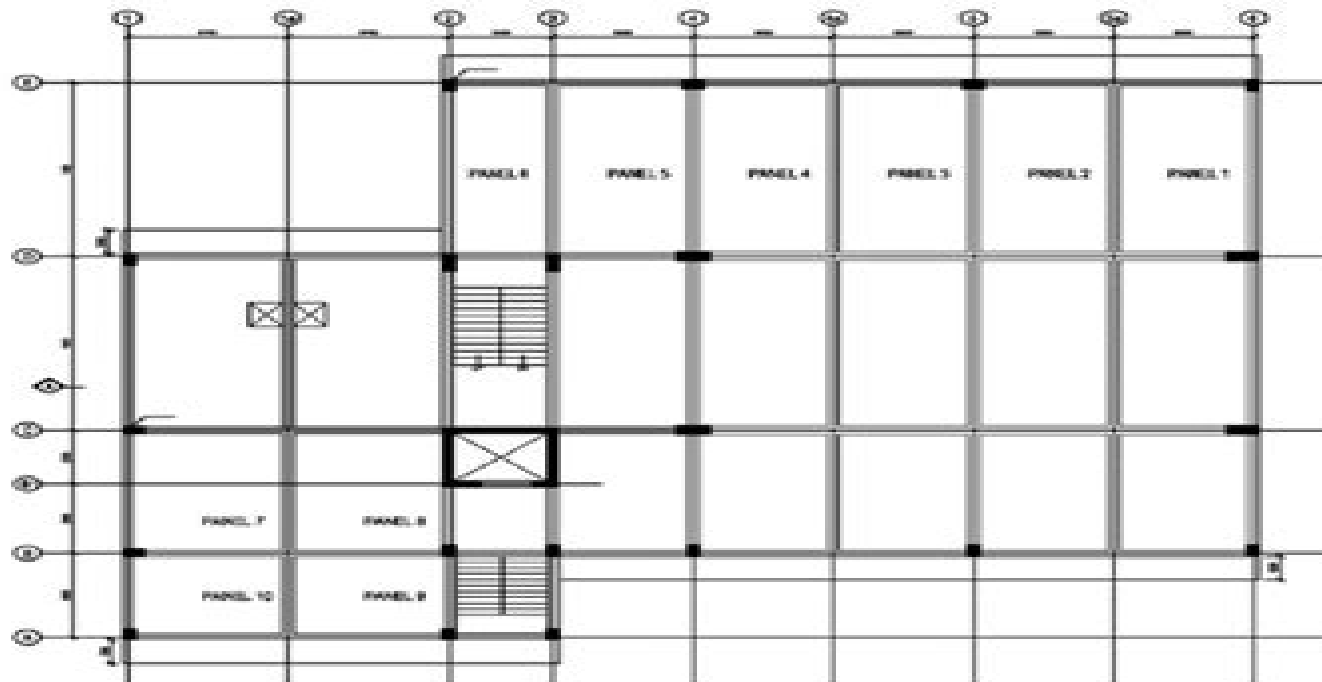
Figure 1.1: General Arrangement
