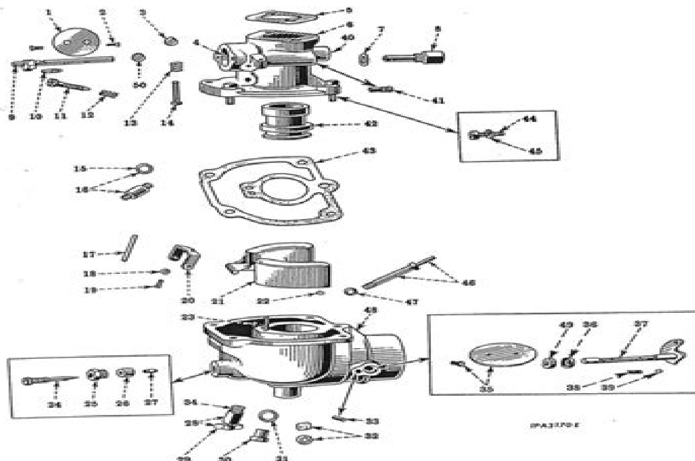
Fig. 6 - Exploded View of International Model E-12, 1-1/4" Updraft and E-13, 1-3/8" Updraft Carburetors.
