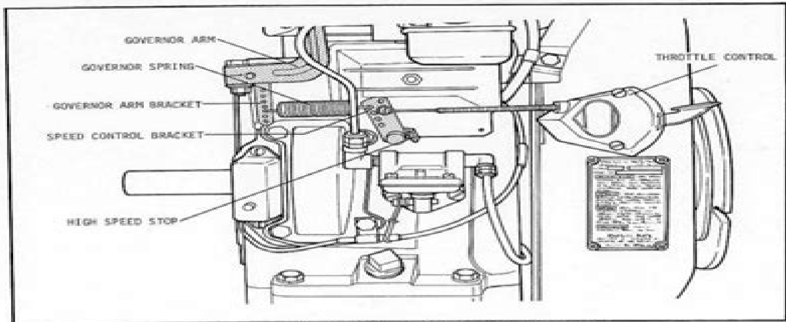
FIGURE 5-5 -- VARIABLE SPEED GOVERNOR - K241, K301, K321
