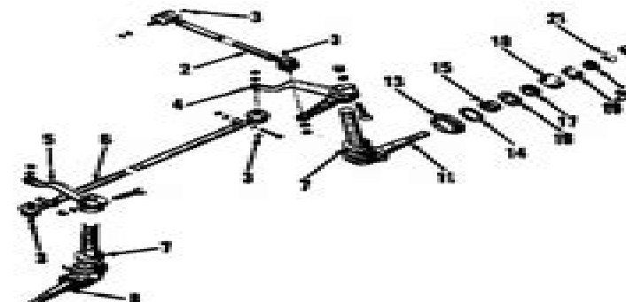
Fig. 7—Exploded view of Series B-275, B-414, 354, 364 and 384 steering knuckles, steering arms, tie rod and drag link used on models with no power steering. Models with power steering are similar.
