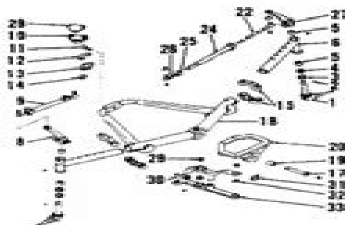
Fig. 5—Exploded view of Series 424, 444, 2424 and 2444 narrow band adjustable front axle and component parts.
