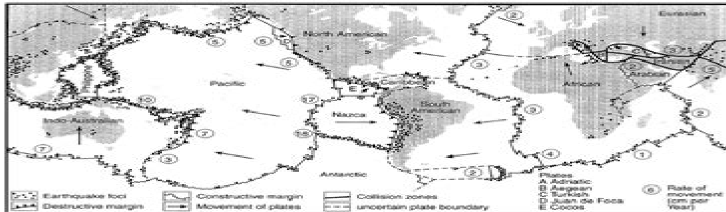
Figure 2: Plate Tectonics: The movement of the crustal plates and the consequence of this movement
