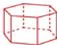
Hexagonal prism
