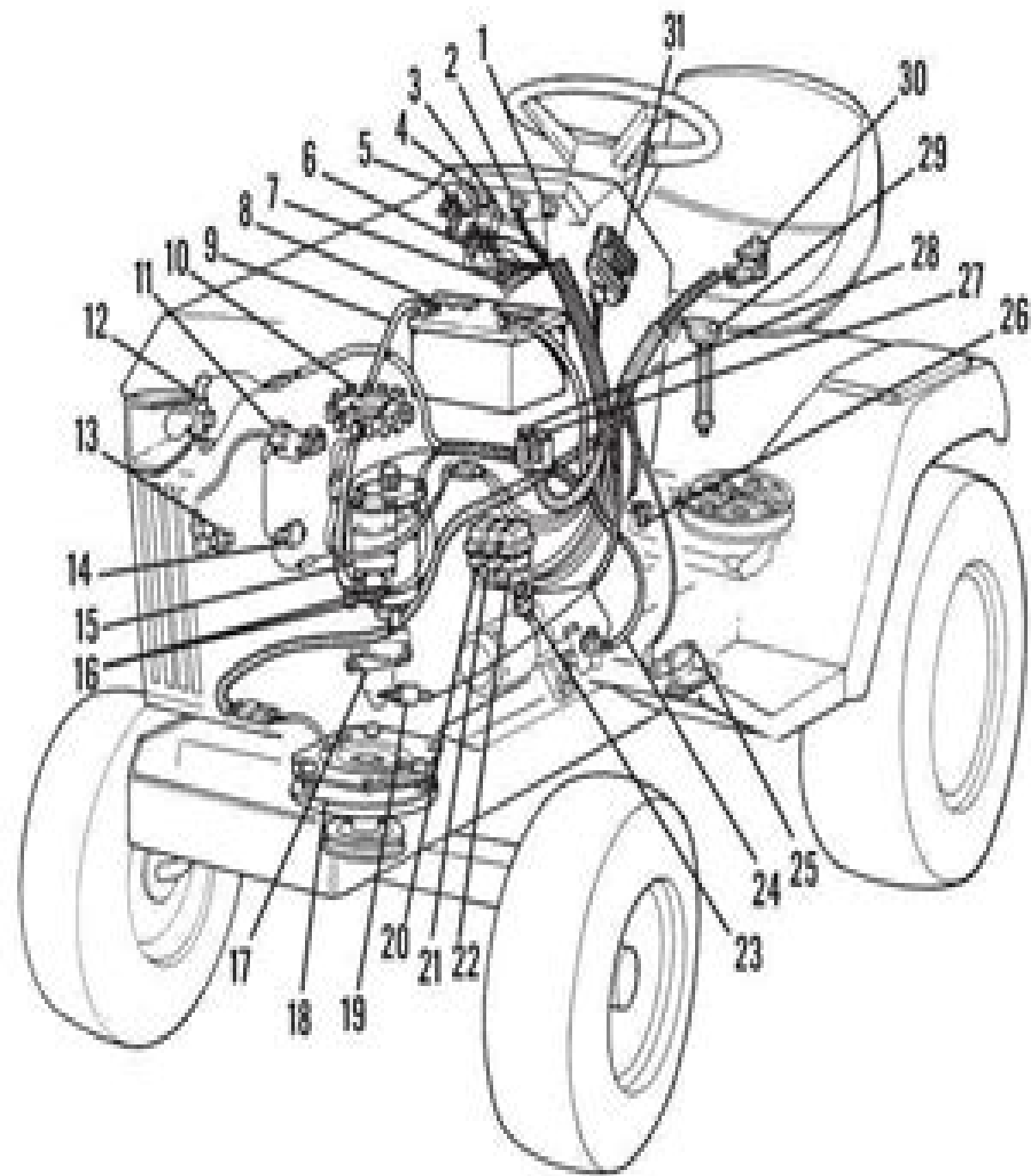
Fig. JD4-18-Drawing showing tractor electrical component location typical for all models.
