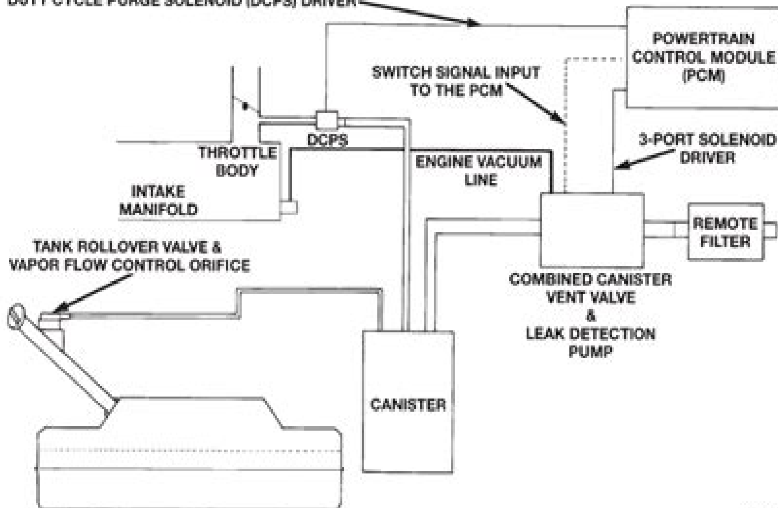
Fig. 4 Evaporative System Monitor Schematic—Typical
