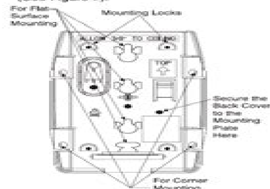
Figure 7. Mounting Plate
