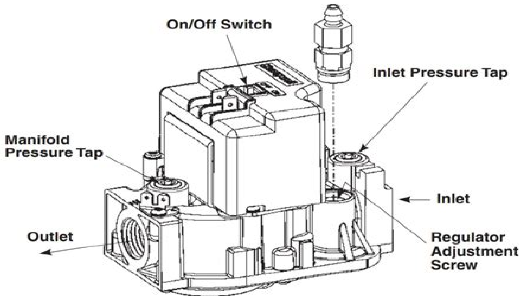
Pressure Regulator Adjustment Screw on Honeywell Gas Valve VR8205
