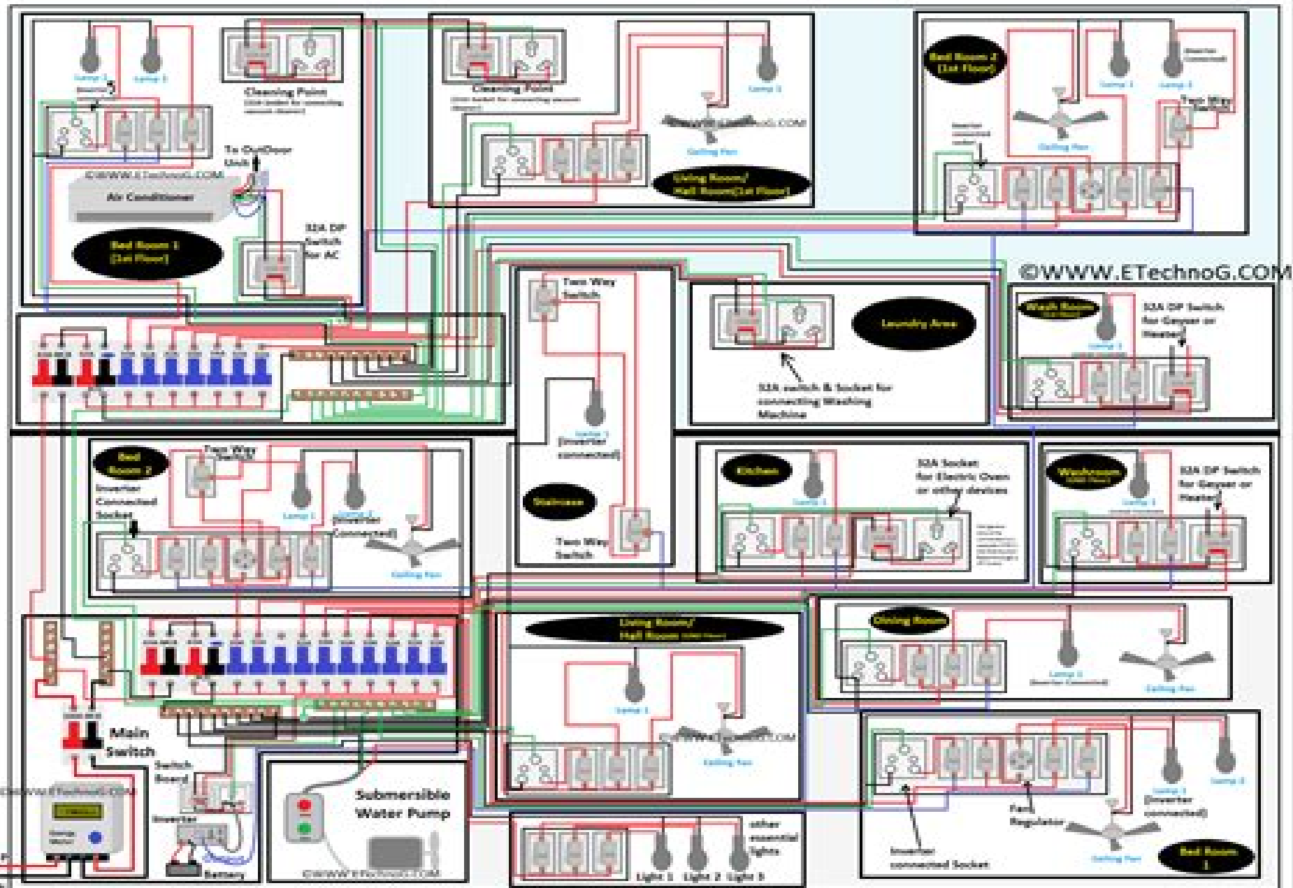
Complete House Wiring Diagram and Connection (Electrical Wiring for a two floor house)
