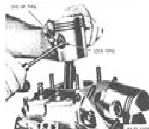
Figure 5—Removing lock ring from piston pin, using tool (91.01.07.01)
