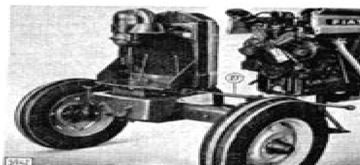
Removing (installing) from axle (640).
