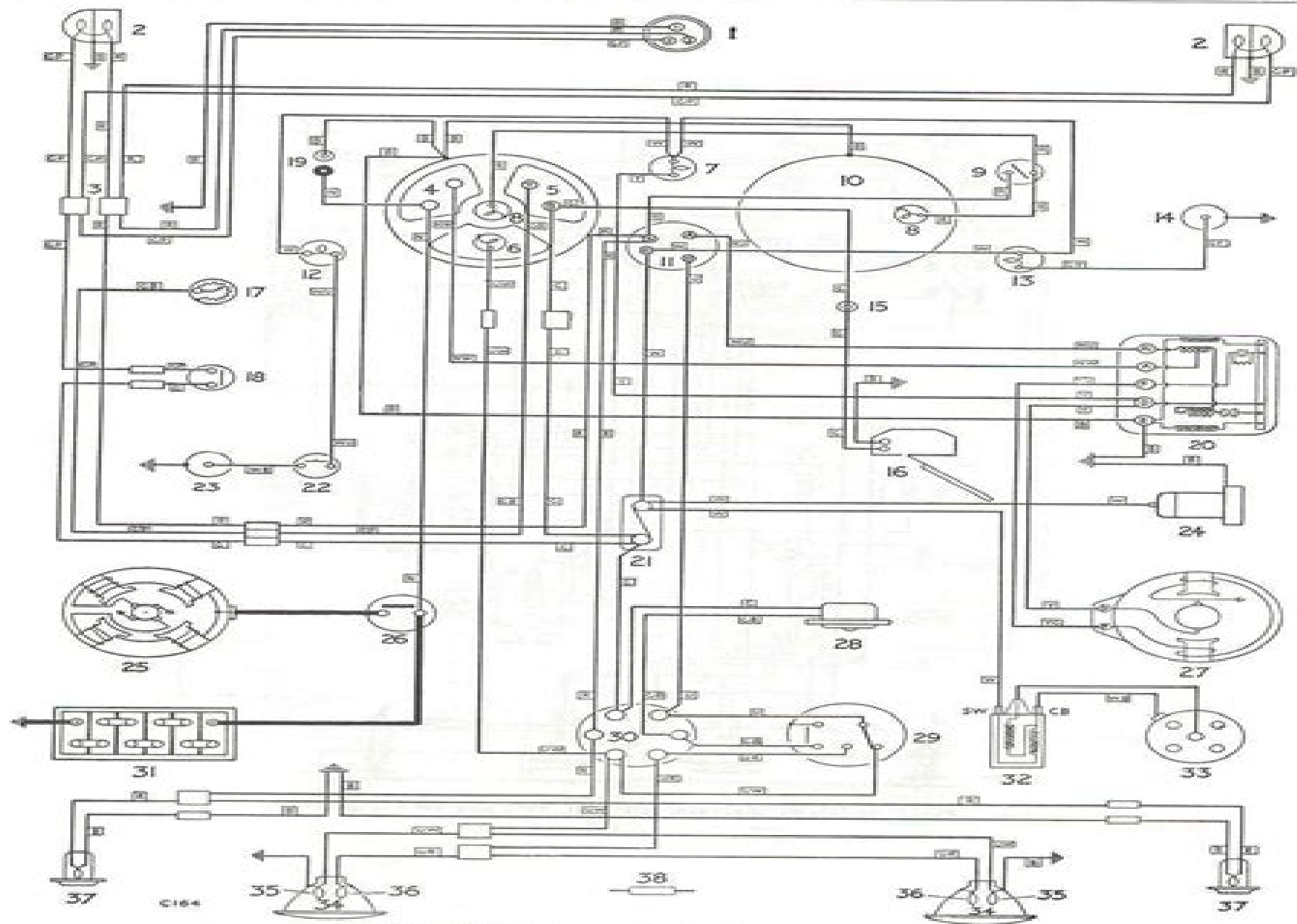
Fig. P-6—Wiring diagram 86 and 107—1956-58 models See Page P-9 for key to wiring diagram
