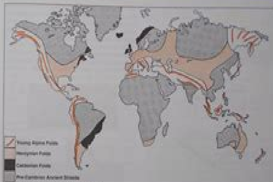
Fig. 17 Structural divisions of the earth.
