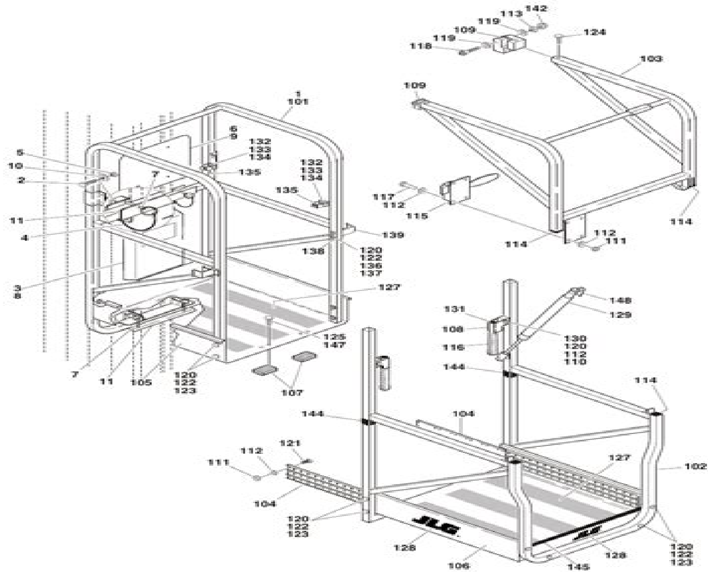
FIGURE 4-4. PLATFORM WITH FRONT ENTRY GULLWING GATE & ROLLING EXTENSION
