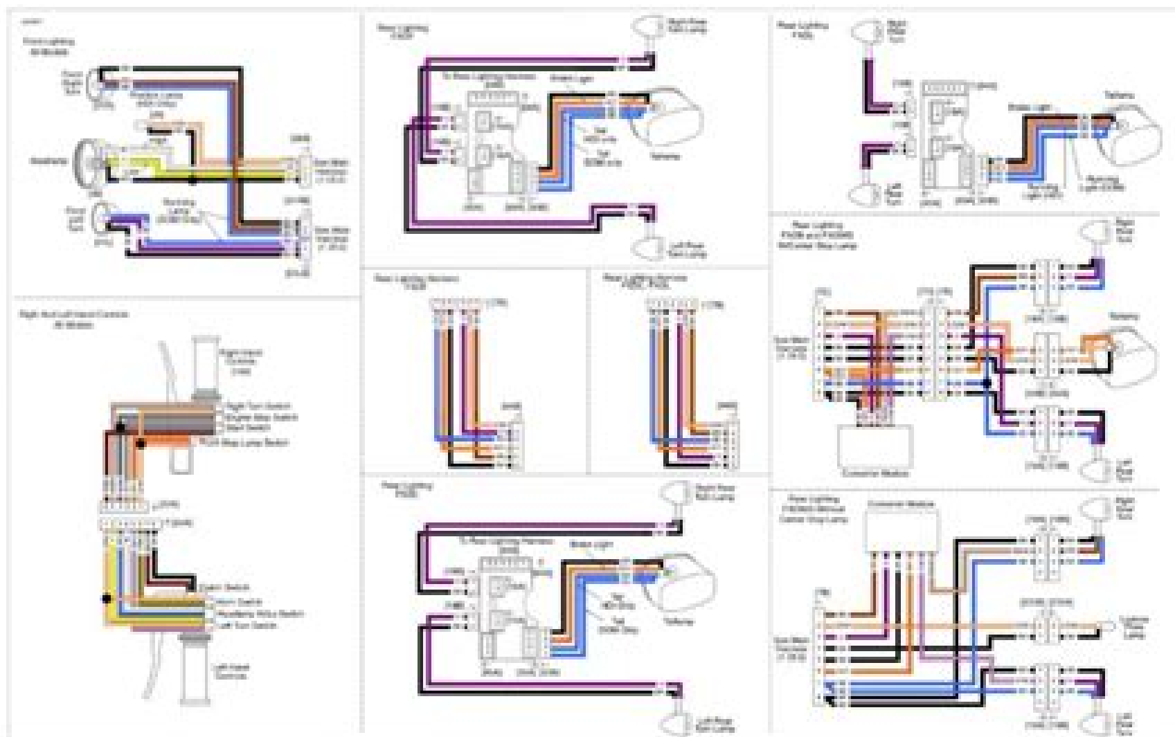
Figure 8-16. Lighting, Horn Controls, and Adapter Harnesses (2011 Style)
