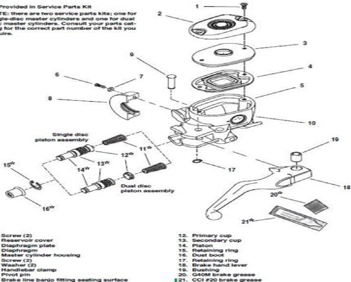
Figure 2-75. Front Brake Master Cylinder Assembly
