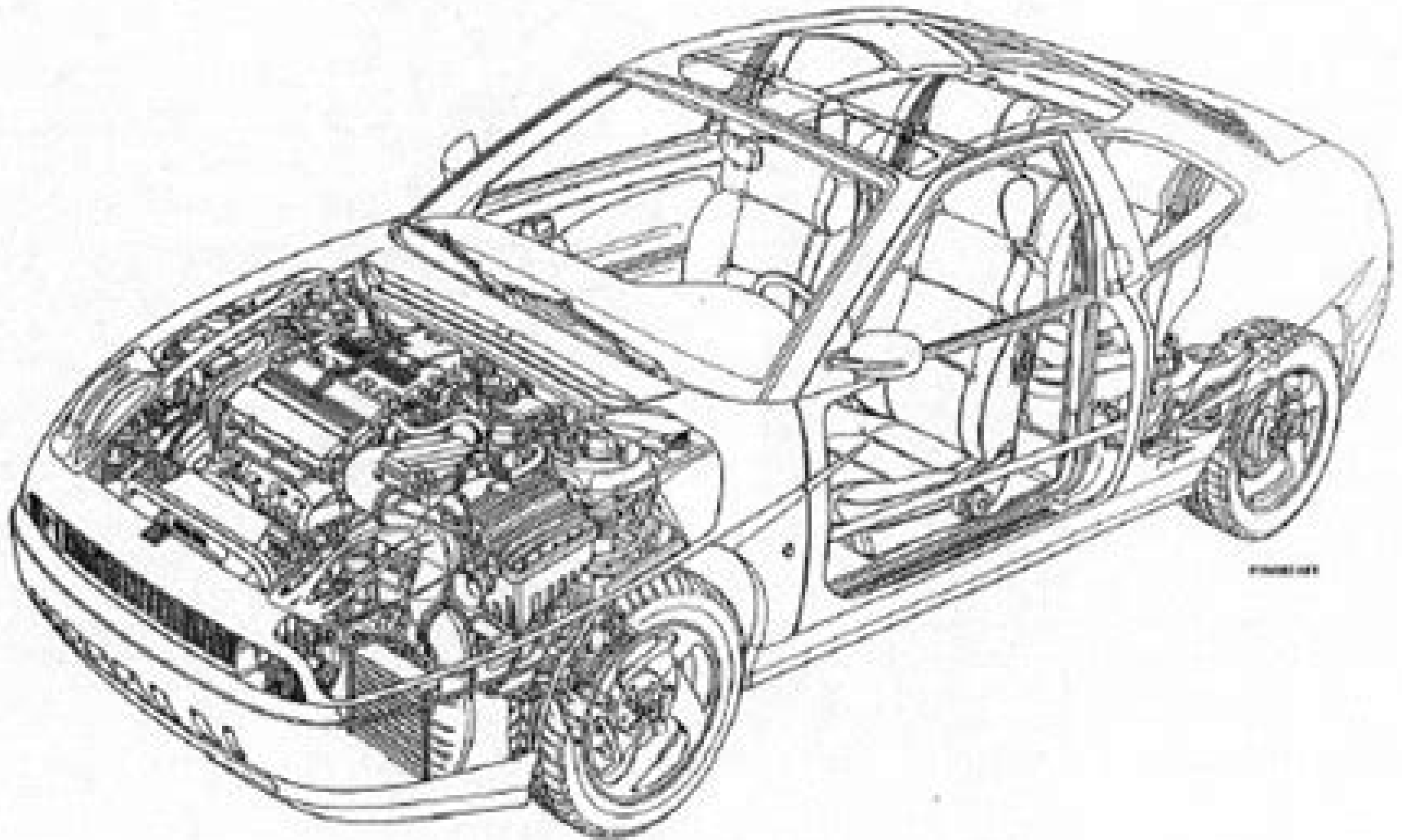
VIEW OF VEHICLE SHOWING LAYOUT OF MECHANICAL COMPONENTS (ENGINE 10Y 6470 )
