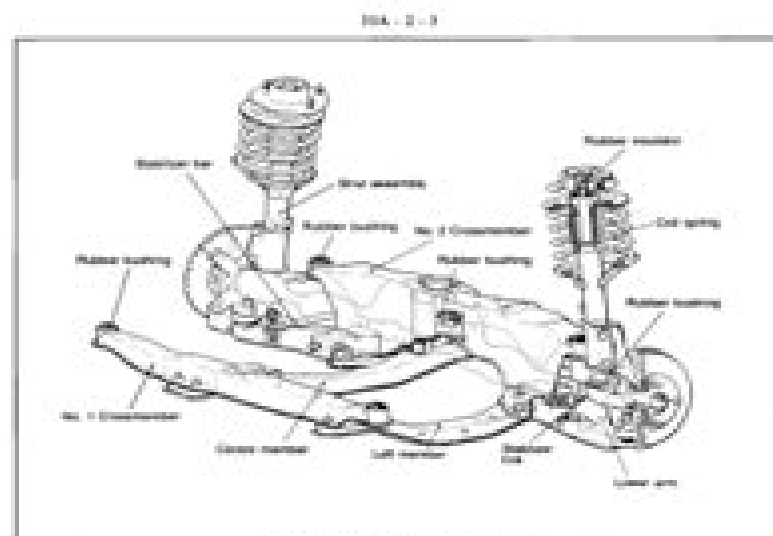
Fig. 1- Front suspension components
