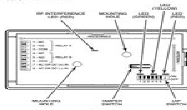
Figure 2. 5800RL Diagram
