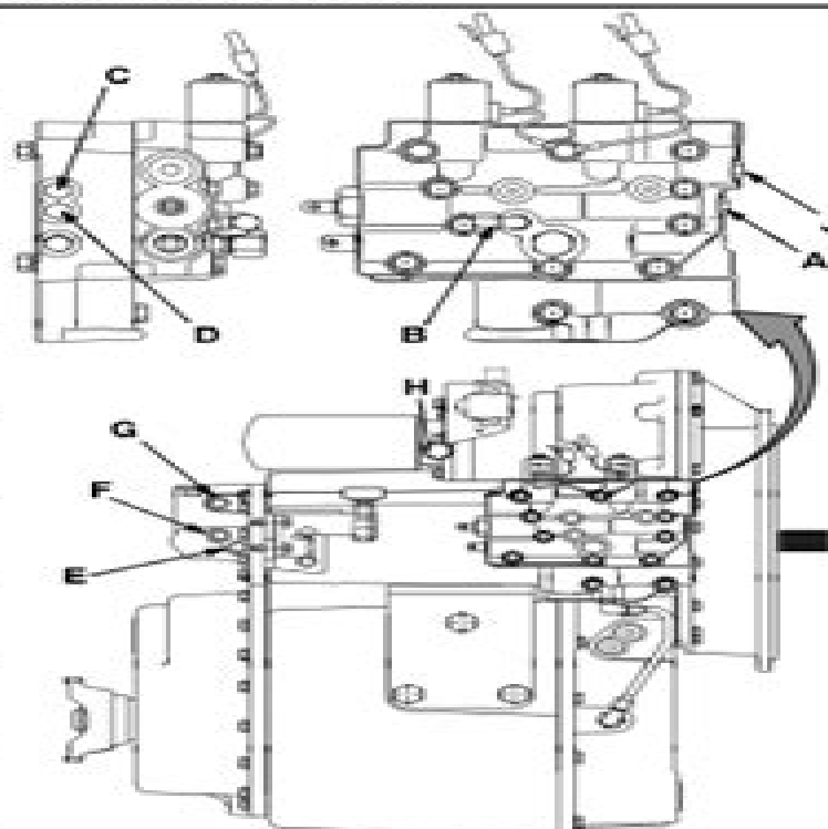
FIGURE 38. TRANSMISSION PRESSURES
