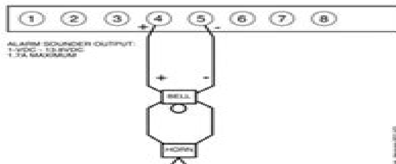
Figure 3-6: Wiring Polarized Fire Devices
