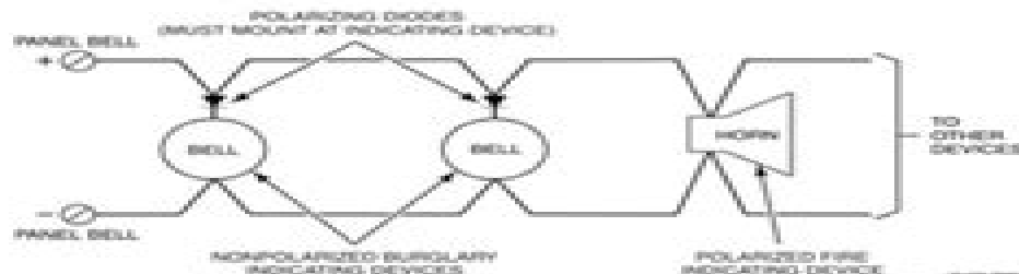
Figure 3-7: Wiring Nonpolarized Burglary Devices
