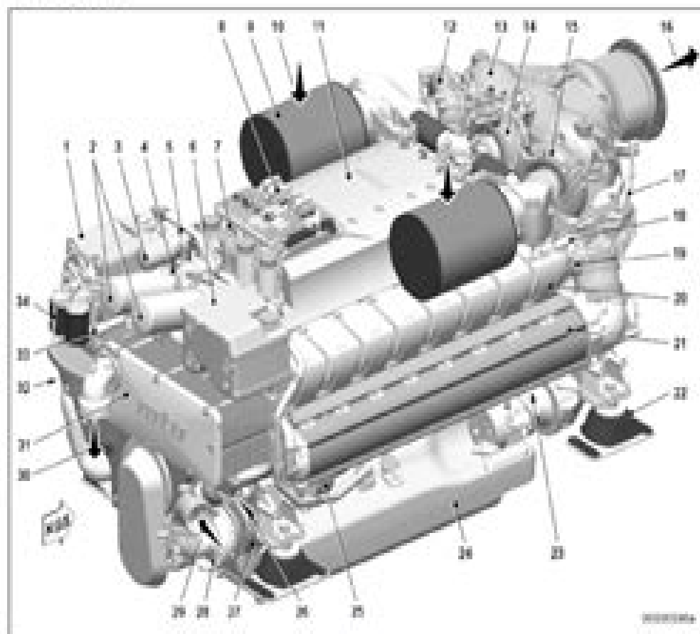
Engine layout
