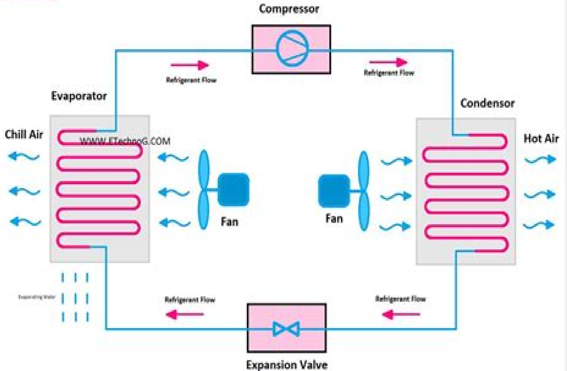
Air Conditioning System Diagram
