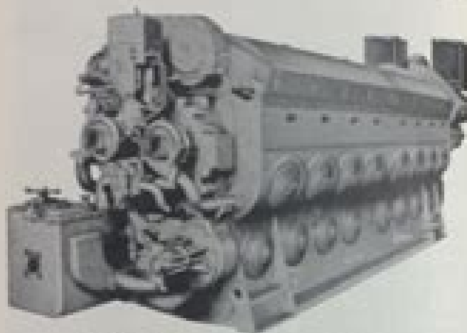
Front Three-Quarter View 160C Engine Fig. 1-2
