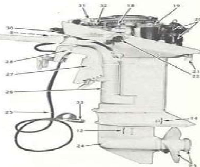
Figure 1-2. Port Side (Electric Start)
