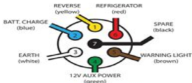
7pin Socket Wiring 12S (Supplimentary)
