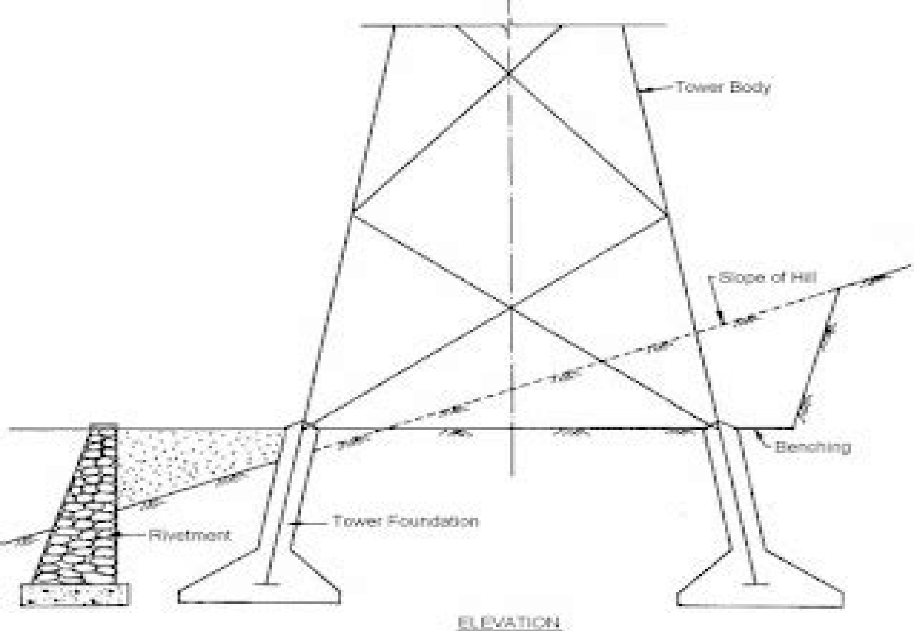
Typical Use of Benching and Rivetment for Protection of Tower Footing
