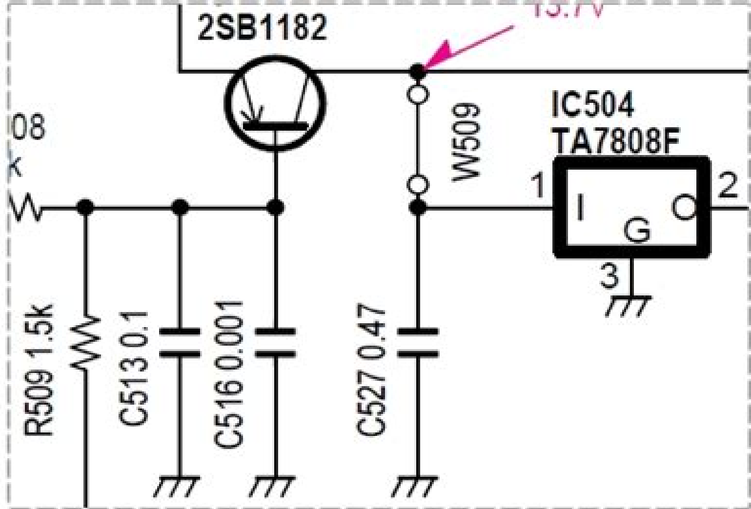
Preview: ICOM IC-208H schematic diagram
