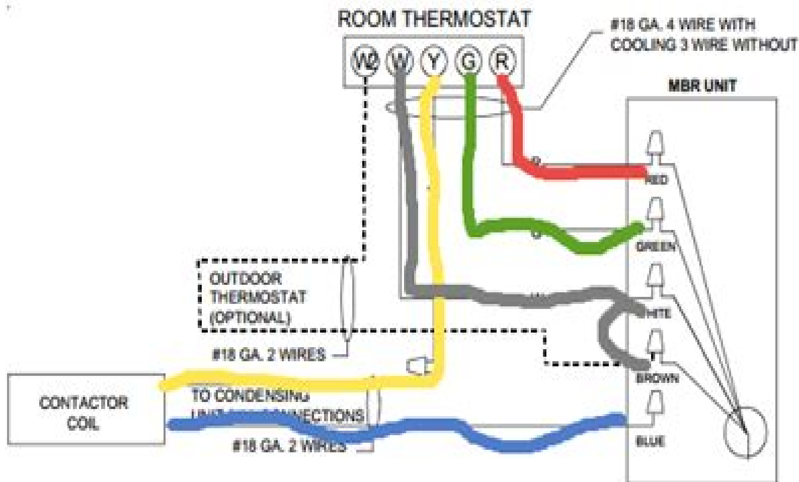
Low Voltage Wiring Diagram for Cooling Unit with optional heat kit 15KW and above
