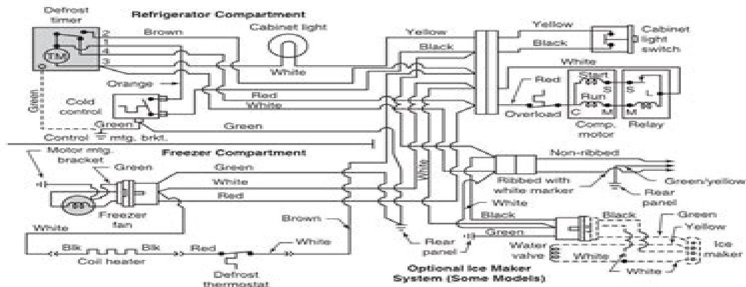
Figure 25-10. A wiring diagram of a typical domestic, single-door automatic defrost refrigerator with a defrost timer and freezer fan. Note color coding of wiring to aid in tracing the circuits.
