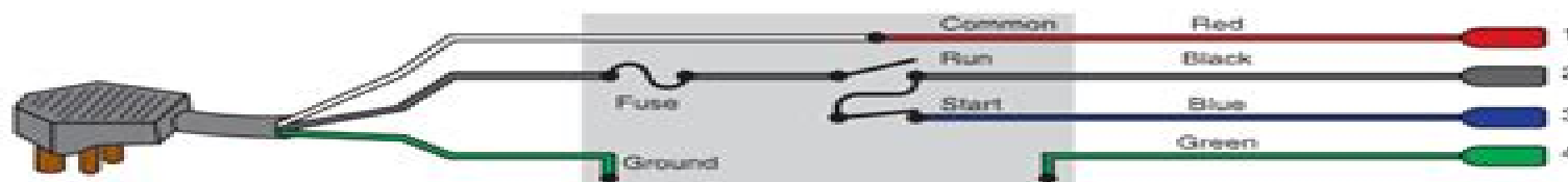
Figure 25-11. A manual start test cord arrangement for hermetic compressors. Clip 1 attaches to the compressor's common terminal. Clip 2 attaches to the run terminal. Clip 3 attaches to the start terminal. Clip 4 attaches to the ground.
