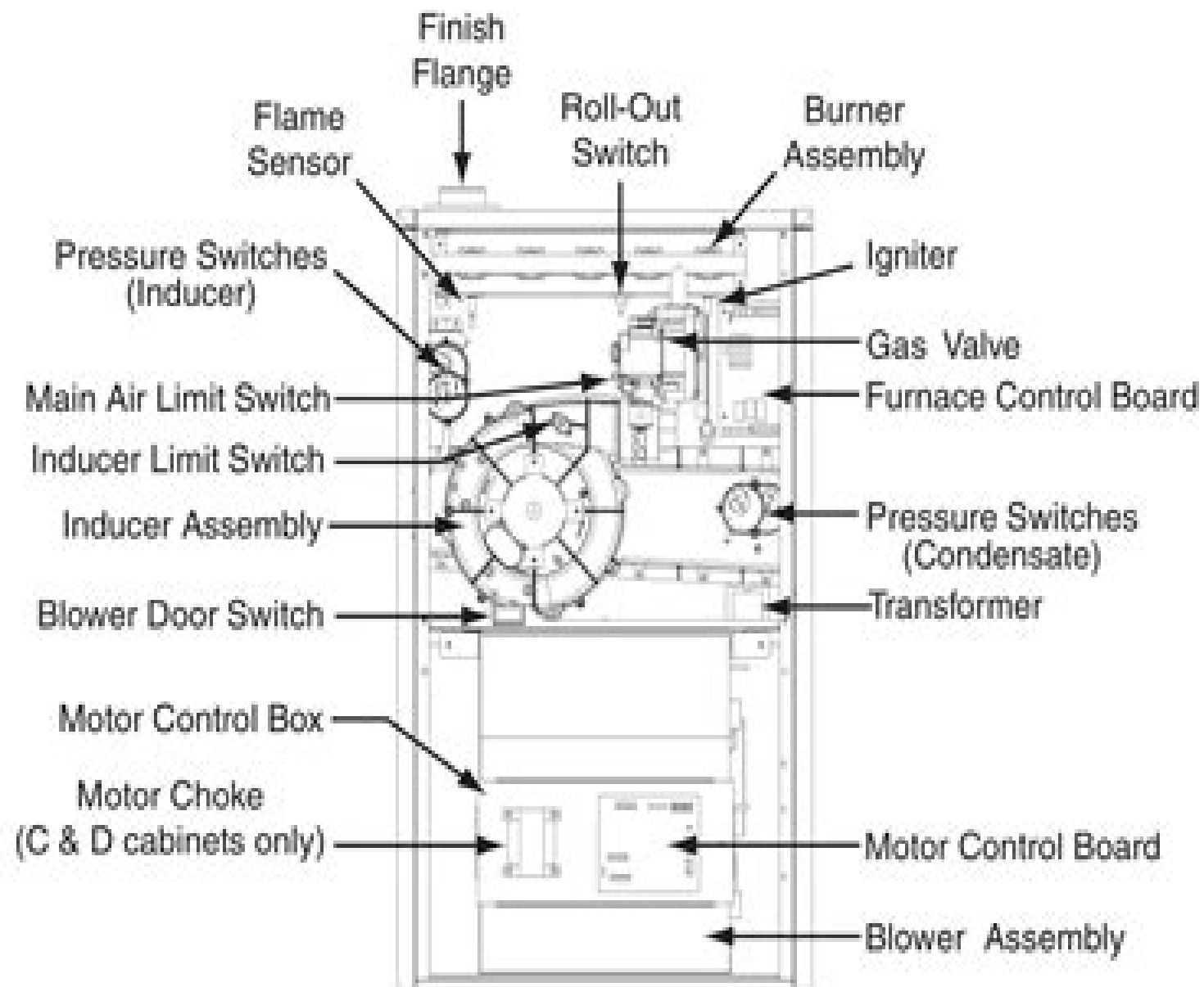
Upflow Gas Furnace Components
