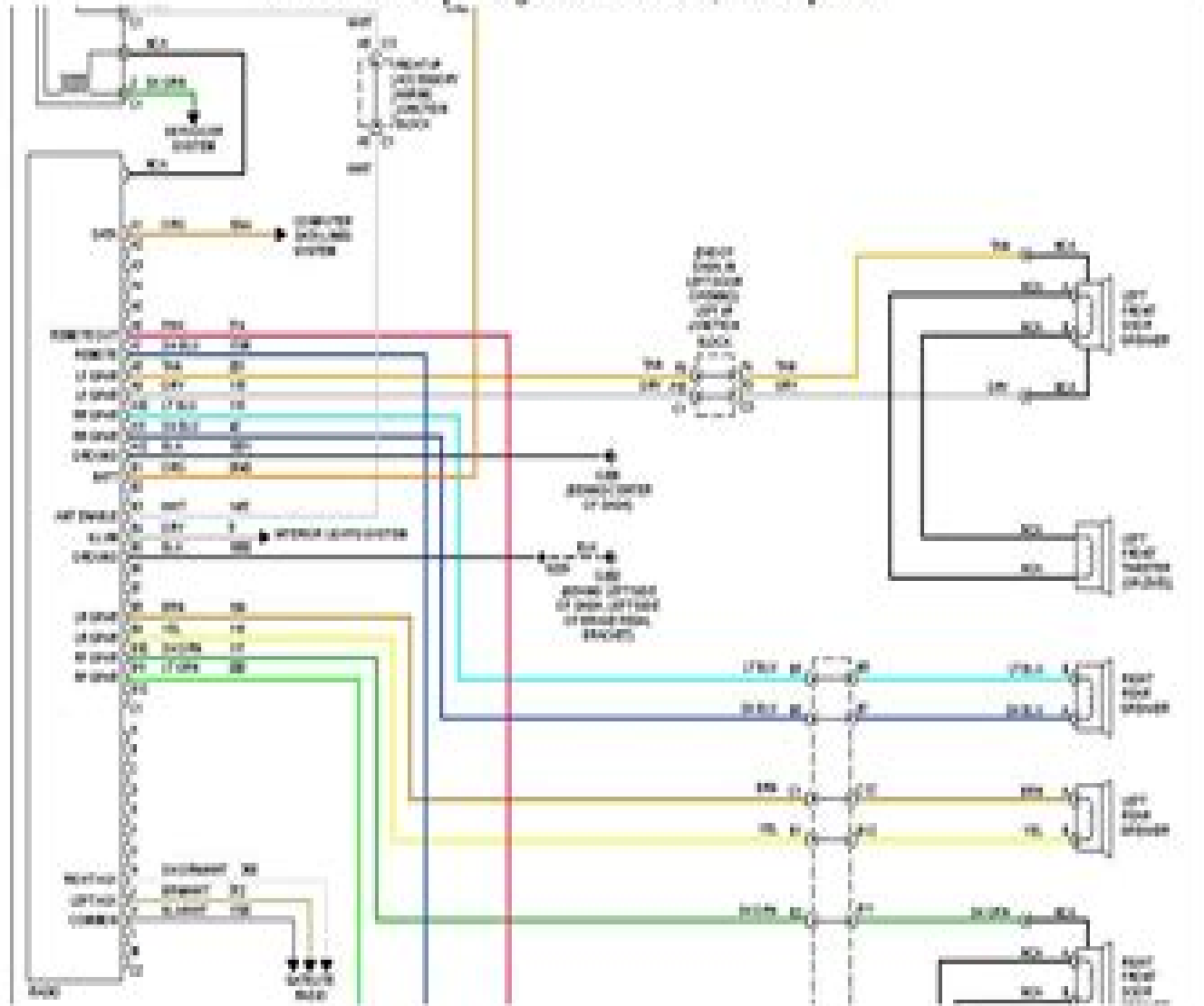
2001 Chevrolet Impala-Fig. 50: Radio Circuit, W/O Amplifier
