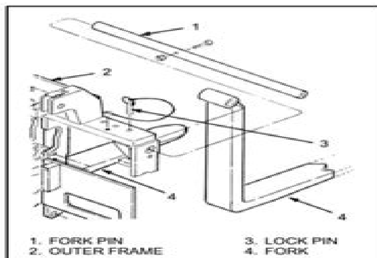
FIGURE 4. FORK REMOVAL
