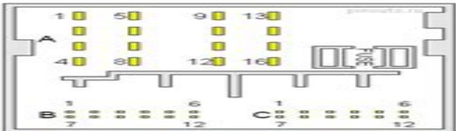
40 (16+12+12) pin QuadLock Fakra Head Unit / Car Stereo connector
