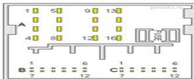
40 (16+12+12) pin QuadLock Fakra Head Unit / Car Stereo connector
