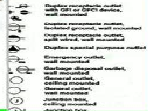
Outlet symbols
