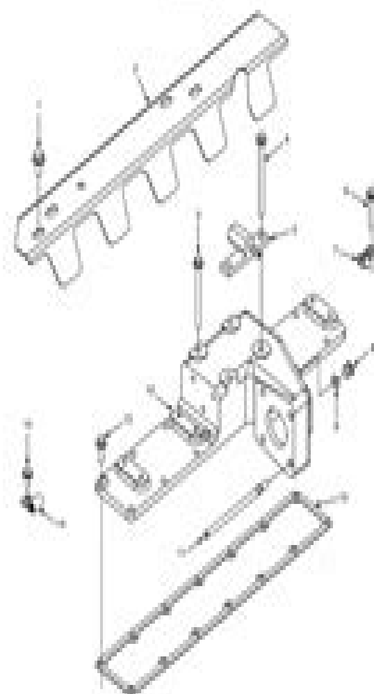
AIR INTAKE CONNECTION FIGURE 3-106 CUMMINS L92
