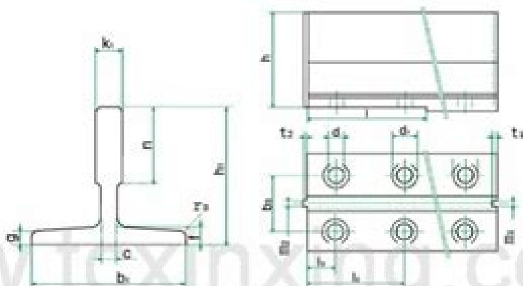
导轨公差尺寸Dimensions and tolerances of guide rails (mm)
