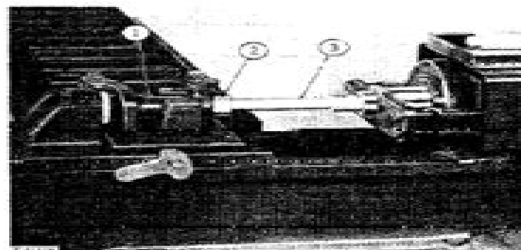
1—Bushings 2—Bushings Forcing Adapter 3—Long Forcing Pin
