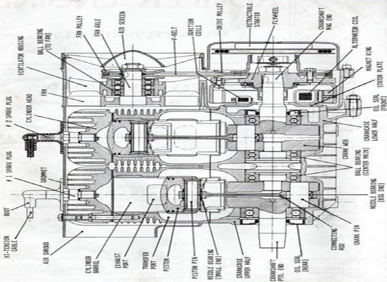
FIGURE 1 -- TYPICAL AXIAL FLOW 2-CYCLE ENGINE
