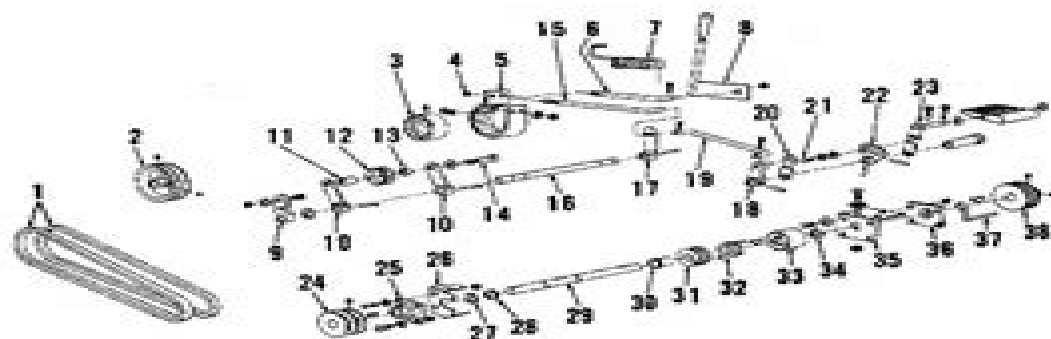
Fig. G11 — Exploded view of clutch-brake system used on Models 754, 755, 780, 53000, 53001 and 53008.
