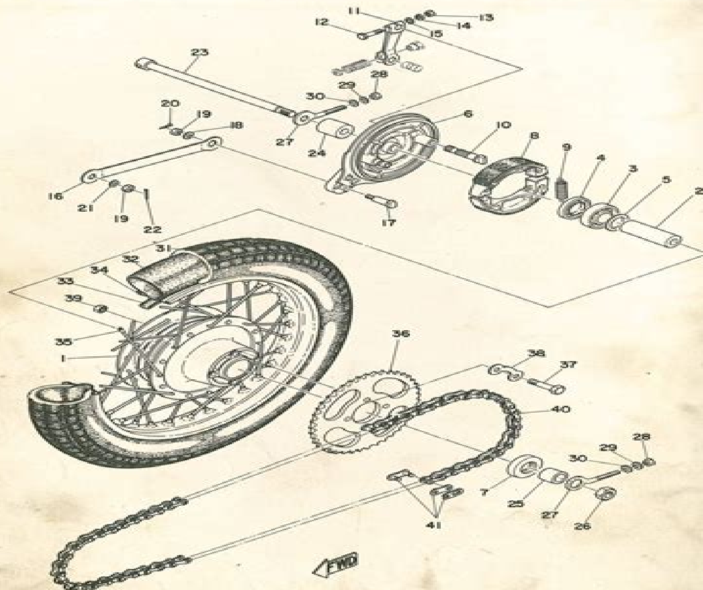
Fig. 24 REAR WHEEL
